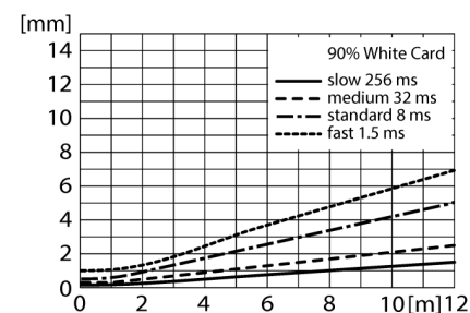
Caracteristica "Excess gain"
