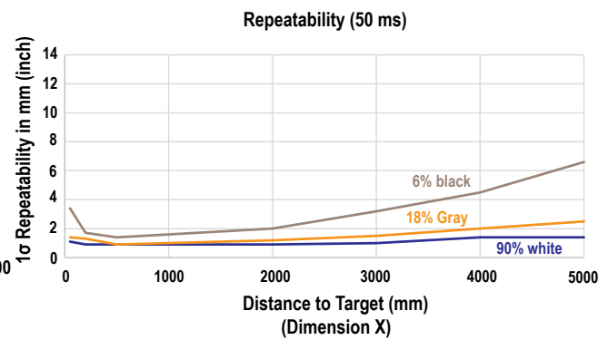
Figure 24. Repeatability for 50 ms Response Time
