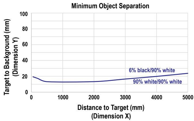
Figure 21. Minimum Object Separation for 250 ms Response Time
