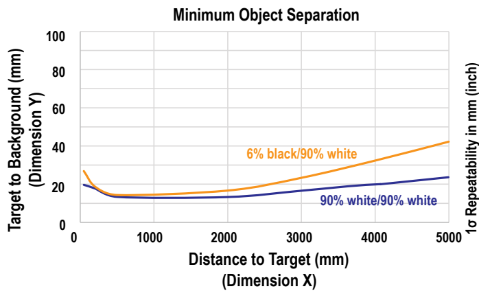
Figure 23. Minimum Object Separation for 50 ms Response Time
