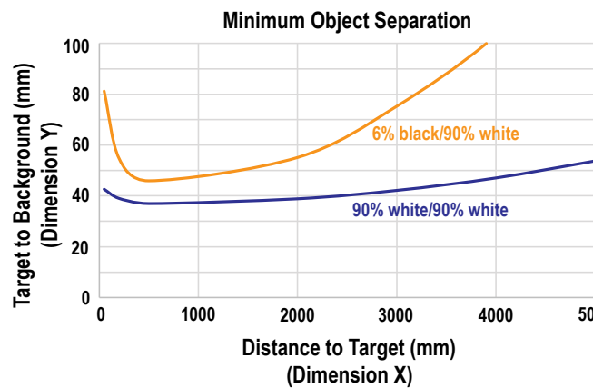
Figure 34. Minimum Object Separation for 5 ms Response Time
