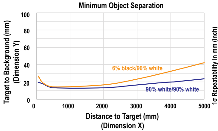
Figure 30. Minimum Object Separation for 50 ms Response Time
