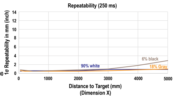
Figure 29. Repeatability for 250 ms Response Time
