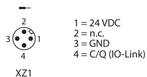
Fig. 4: Pin assignment
