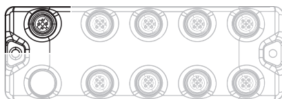
Fig. 3: M12 connector for the connection to an IO-Link master
