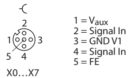
Fig. 6: Pin assignment TBIL-EMN-16DIP (X0...X7)
