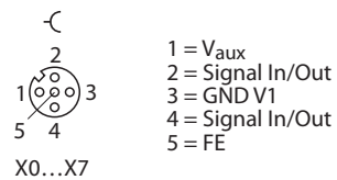
Fig. 7: Pin assignment TBIL-EMN-16DXP (X0...X7)
